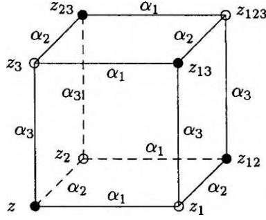
Figure 3. Elementary cube
